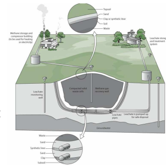
Figure 17.7 Generalized Depiction of a State-of-the-Art Sanitary Landfill (Cited from Frumkin's text)
