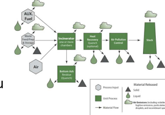
Figure 17.8 Generalized Diagram of Incineration Material and Process Flow
