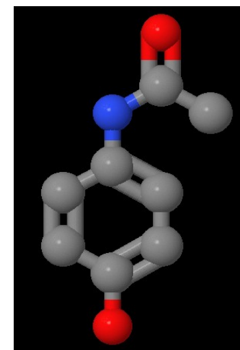
500 mg/kg (acetoaminophene)
