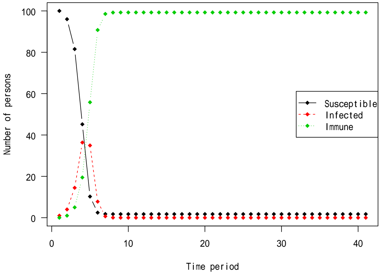
Reed-Frost projection of epidemic curve where p=0.04
