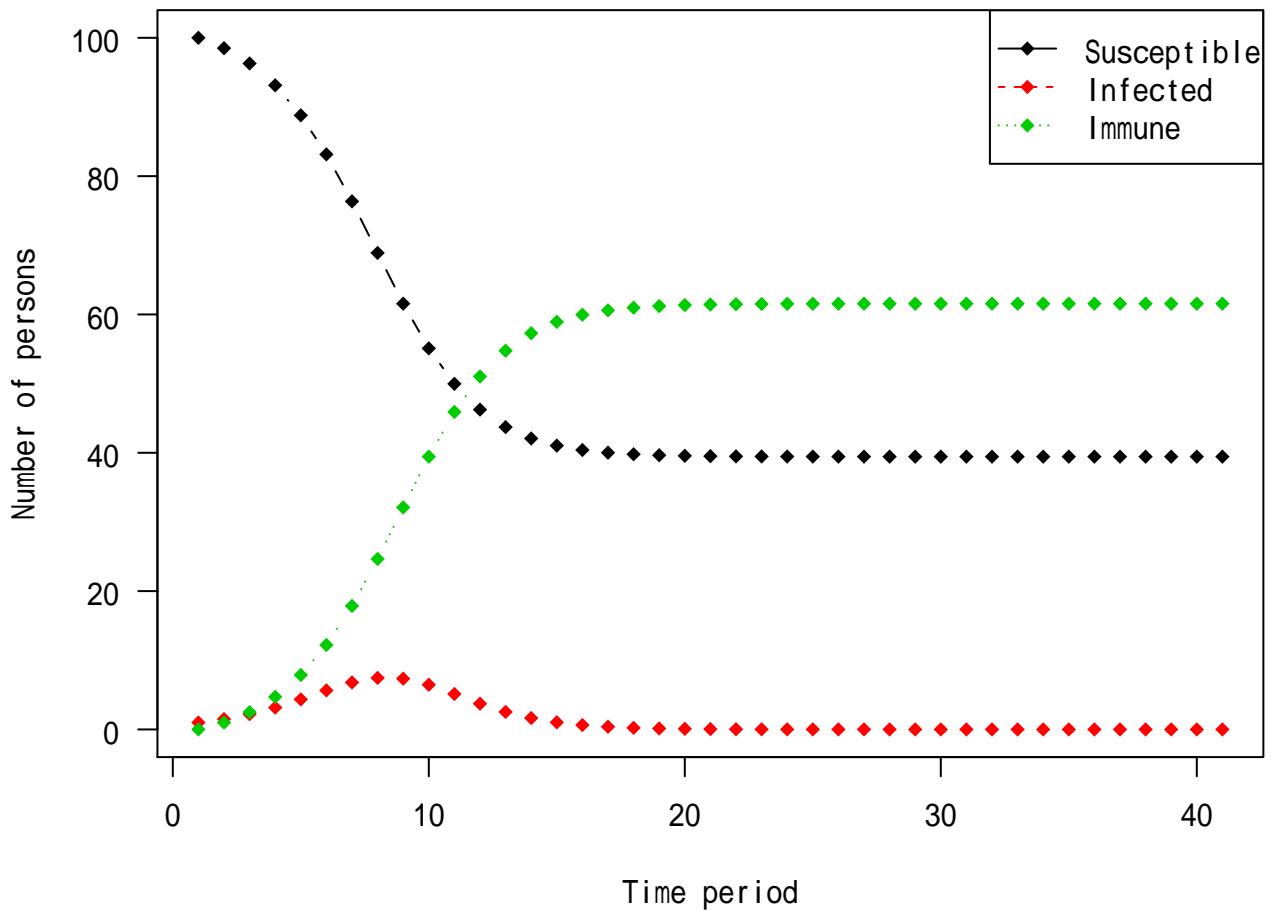
Reed-Frost projection of epidemic curve where p=0.015
